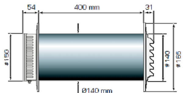
Dimensions Fresh 90-dB, Ø140mm
