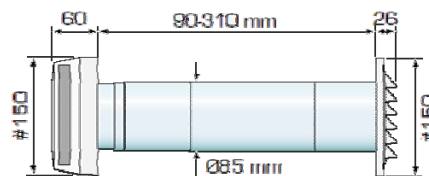
Dimensions TL80P
