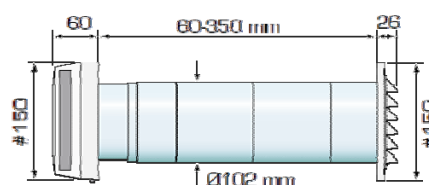
Dimensions TL98P
