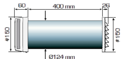
Dimensions TL80P-dB, TL98P-dB
