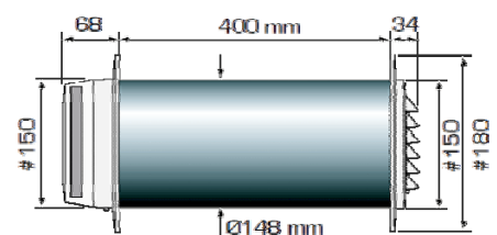
Dimensions TL80P-dB, TL98P-dB
